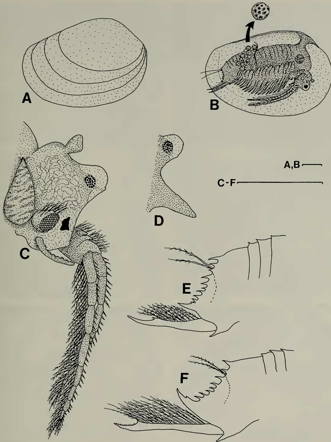
Fig. 1. Eulimnadia ovilunata : A, Right valve of holotype female; B, Holotype female, right valve removed, with egg enlarged above; C, Frontal region of holotype female; D, Rostrum and eye of one of three poorly preserved males; E, Caudal region of holotype female; F, Caudal region of male. Scale bars indicate 1.0 mm.
